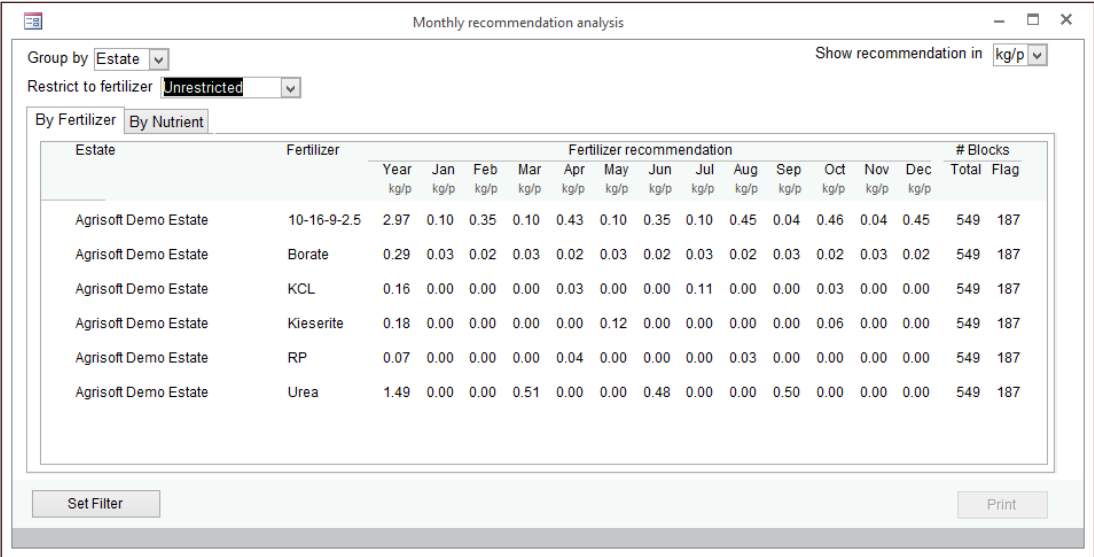
Figure 3. Example of CDST output, in this case summarizing application rates (kg/palm) for an estate.
